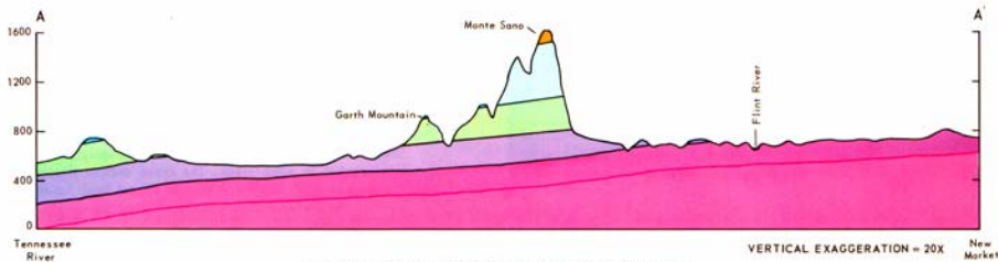
CROSS SECTION SHOWING RELATIONSHIP OF ROCK UNITS
